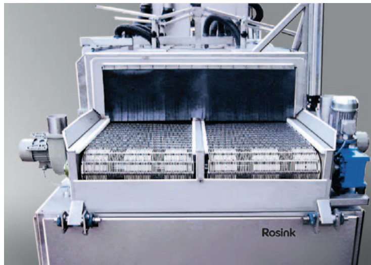
Twin belt system for stampings and deep drawn parts for loads of up to 100kg/m
