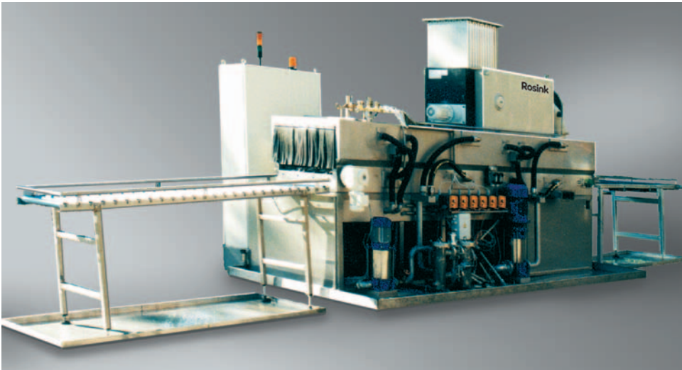
Top: System with feed and discharge system for cleaning and drying of sawn timber sections with mechanical condensation stage Bottom: Continuous cleaning system with feed and discharge system for cleaning and drying of cut aluminium parts
